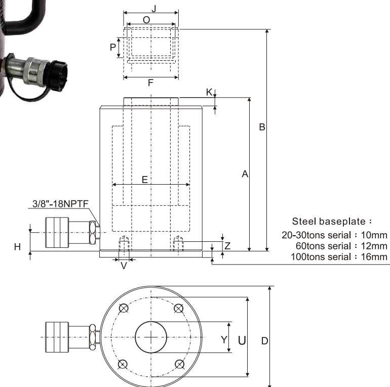
缸底墊塊底座螺孔 Steel Base Plate Mounting Holes
